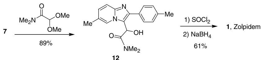
Scheme 15.2. Industrial-scale synthesis.
