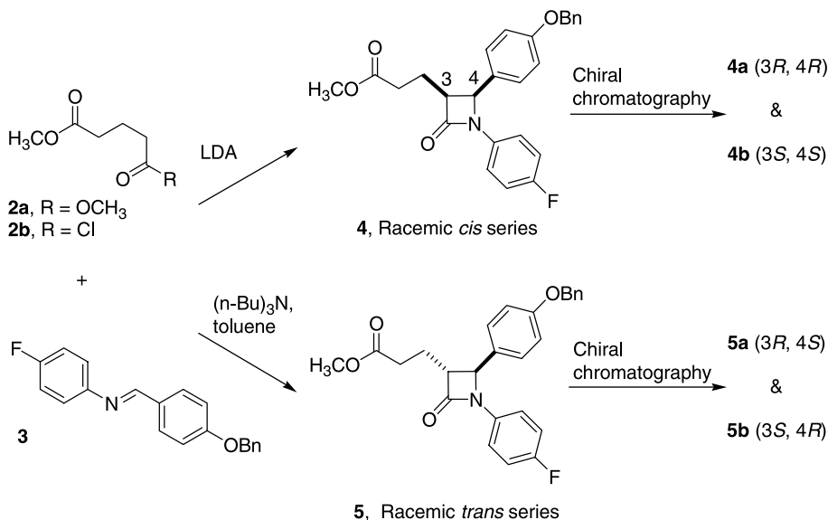
Scheme 13.1.
