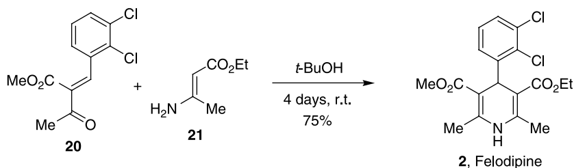
Scheme 11.2. Synthesis of felodipine ( 2 ).
