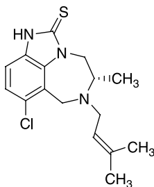
Figure 6.1. R86183.
