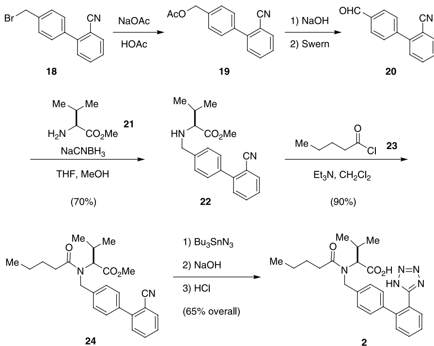
Scheme 9.5. The Novartis/Ciba-Geigy synthesis of valsartan ( 2 ).
