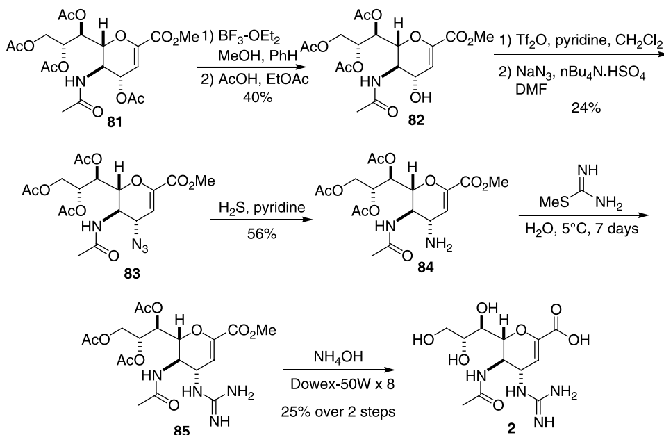
Scheme 7.12. The Biota synthesis of zanamivir ( 2 ) from the patent literature.
