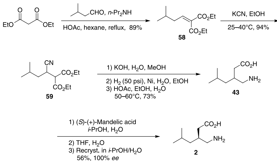
Scheme 16.16. The malonate approach to pregabalin ( 2 ).
