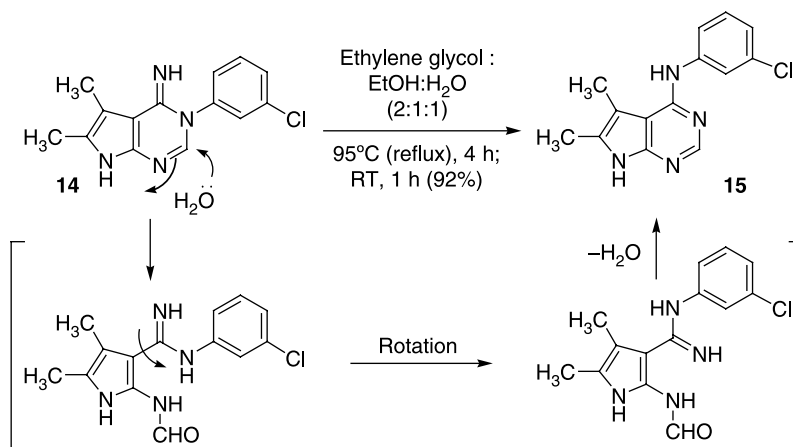
Scheme 2.4. Process for preparing a pyrimidine by Dimroth “rearrangement.”
