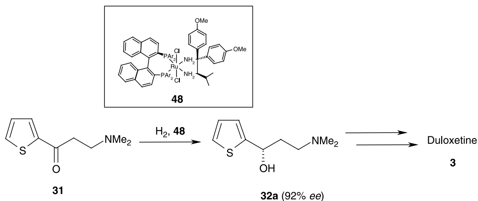
Scheme 14.15.
