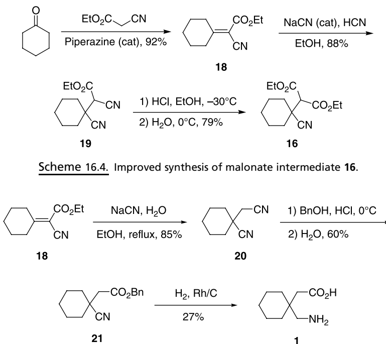
Scheme 16.5. Mettler's synthesis of gabapentin (1).
