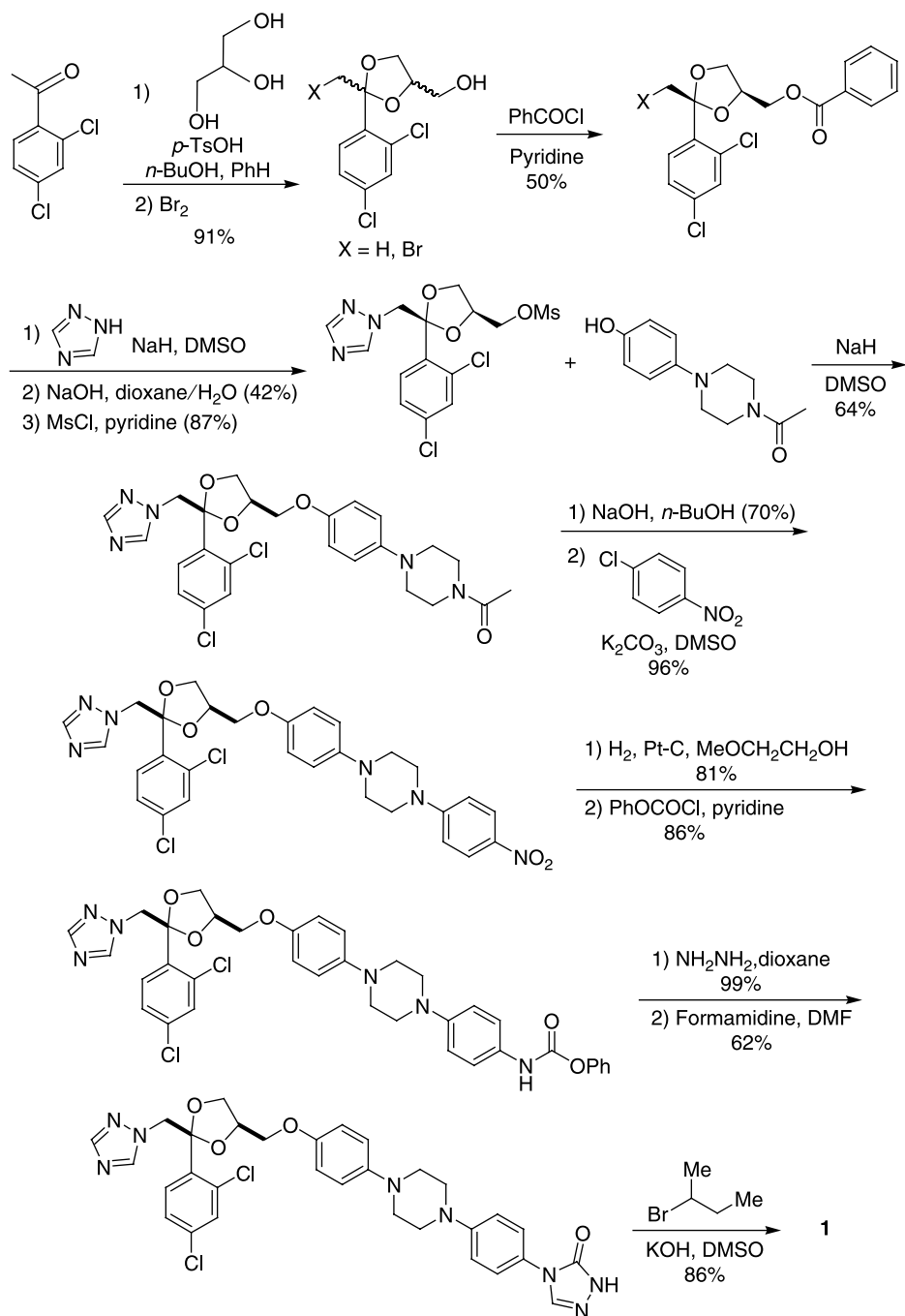
Scheme 5.2. Synthesis of itraconazole (1).
