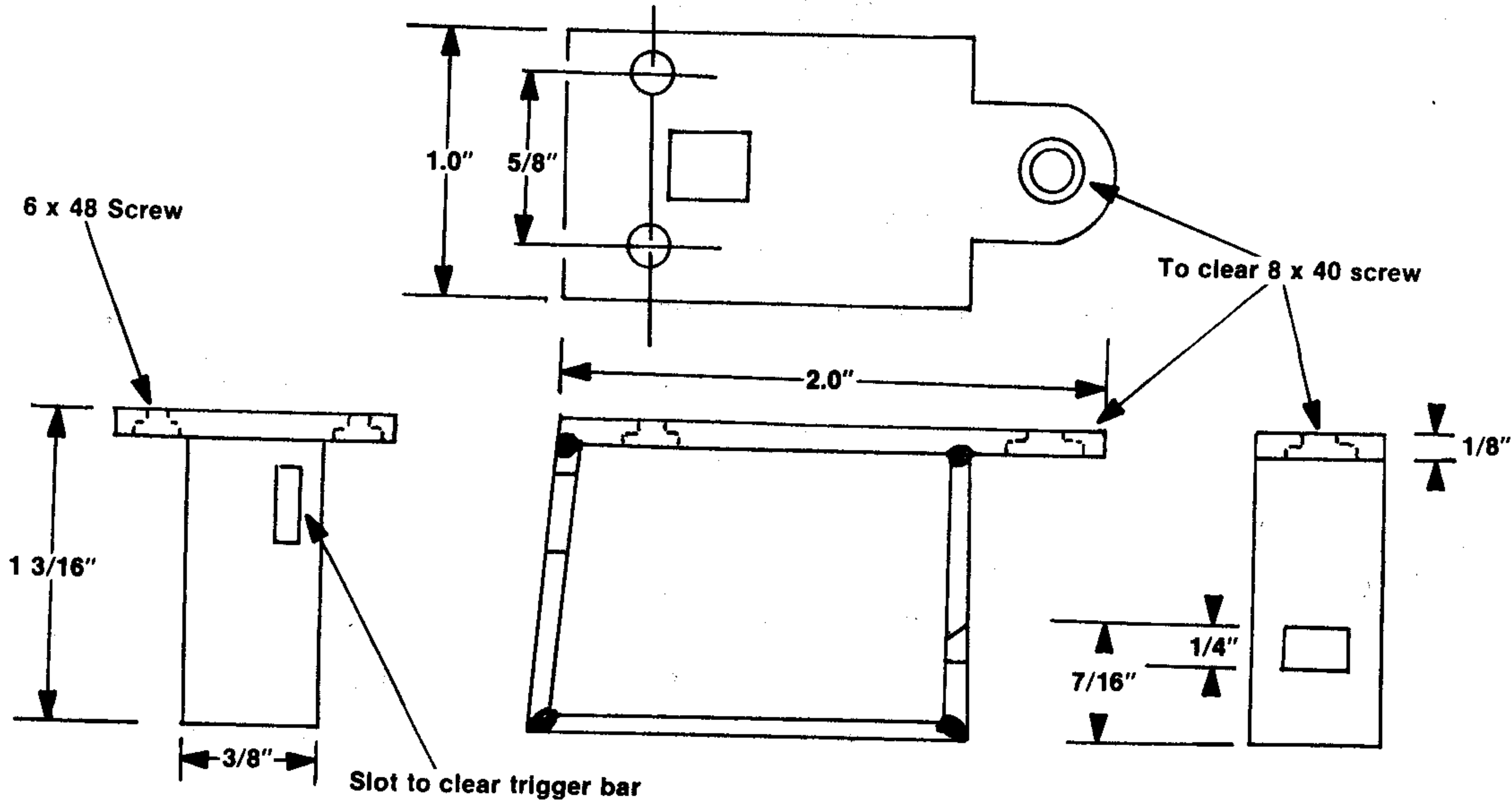
TRIGGER GUARD
