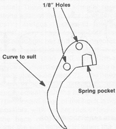
TRIGGER
