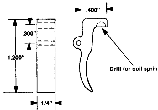
TRIGGER
