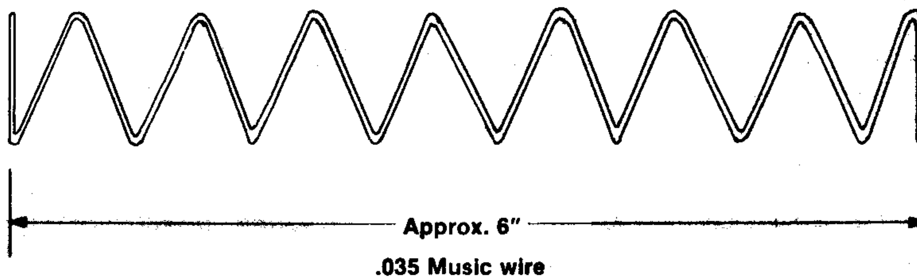
MAGAZINE SPRING
