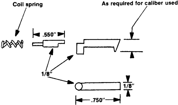
EXTRACTOR
