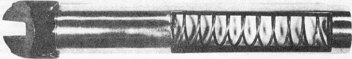
Above: top view of the finished slide assembly with home-built recoil spring in place.
