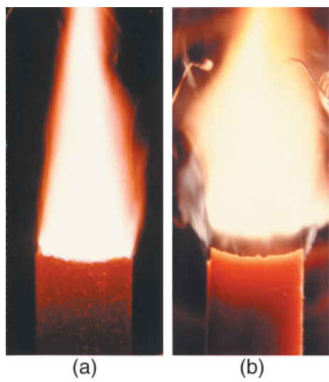
Figure 7-31. Flame structure of AP-CMDB propellant.
