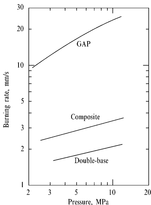
Figure 9-23. Burning rate characteristics of gas-generating propellants.
