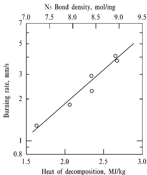
Figure 5-15. Burning rate of BAMO copolymer increases with increasing heat of decomposition and also with increasing N 3 bond density.
