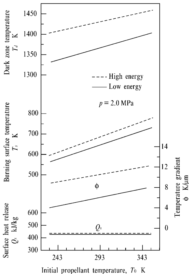
Figure 6-16. Dark zone temperature, burning surface temperature, surface heat release, and temperature gradient in the fizz zone of high- and low-energy double-base propellants as a function of initial propellant temperature.
