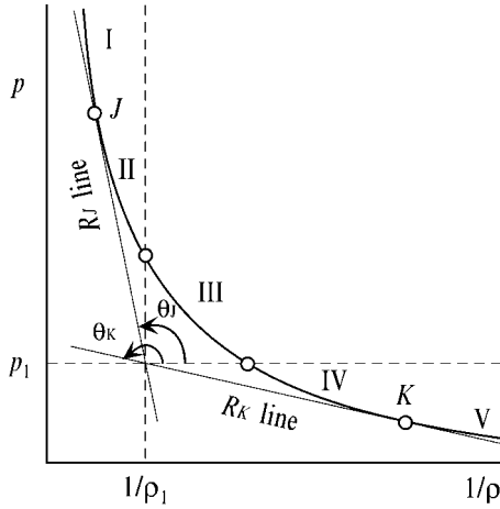
Figure 3-3. Definition of Hugoniot curve for combustion wave.
