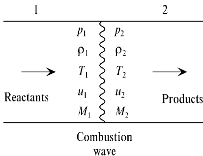
Figure 3-1. Combustion wave propagation.
