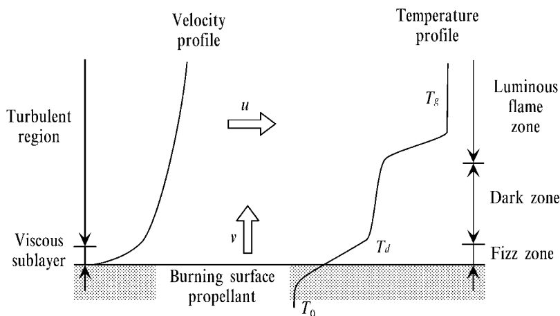
Figure 9-12. Erosive burning effect on the flame structure of double-base propellant.
