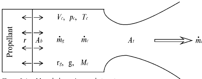
Figure 9-4. Mass balance in a rocket motor.
