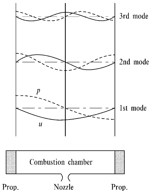
Figure 9-20. Combustion mode in T burner.
