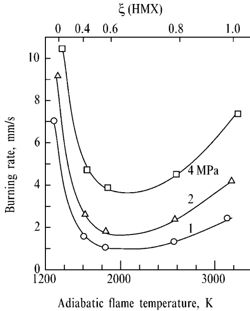
Figure 7-21. Burning rate of HMX composite propellant as a function of adiabatic flame temperature or \xi (HMX) showing the existence of the minimum burning rate at about \xi(0.6) .
