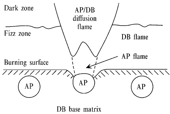
Figure 7-31. Flame structure of AP-CMDB propellant.
