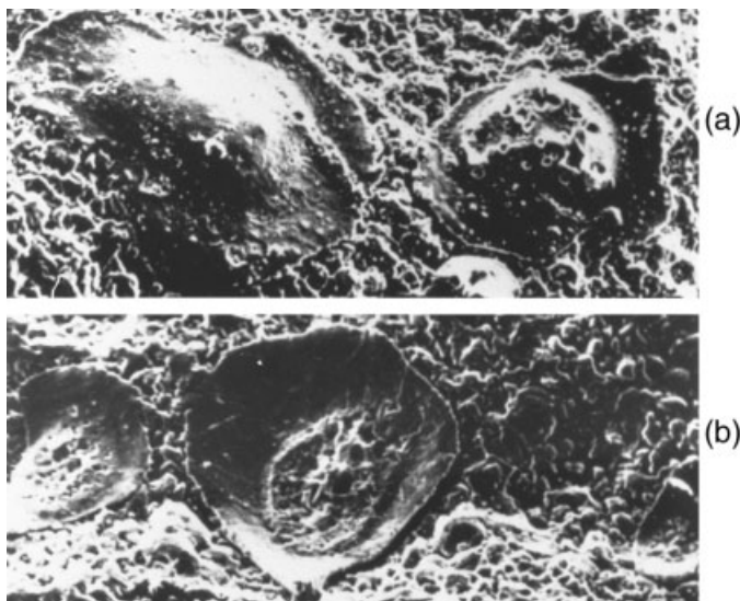
Figure 7-15. Scanning electron microphotographs of quenched AP composite propellant burning surfaces without LiF (a) and with 0.5 % LiF (b) obtained by a pressure decay from 2 MPa to 0.1 MPa; the width of each photograph is 0.60 mm.
