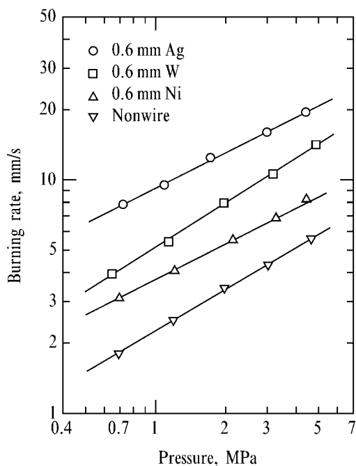
Figure 9-14. Effect of metal wire on burning rate along the wire.
