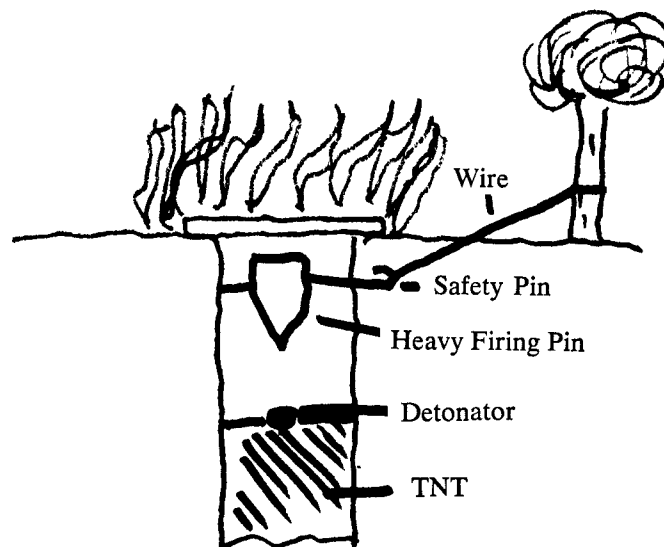
Figure 101. Walk trap.
