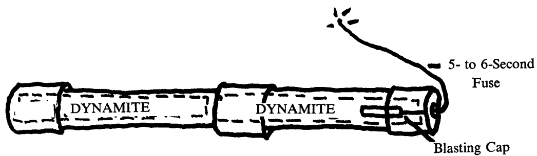
Figure 102. Bangalore torpedo.
