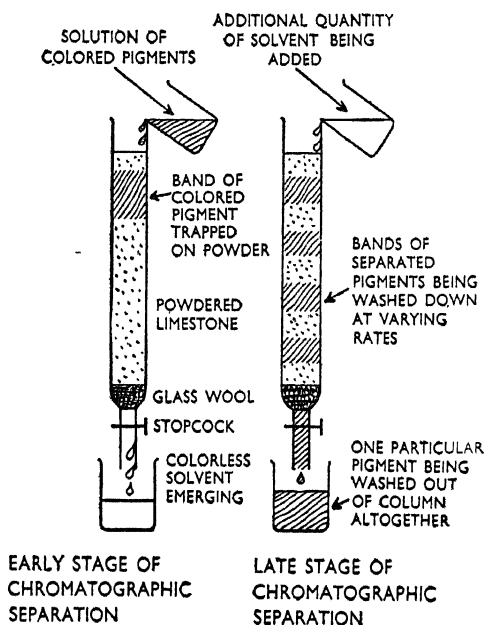
Figure 10. Column chromatography.
