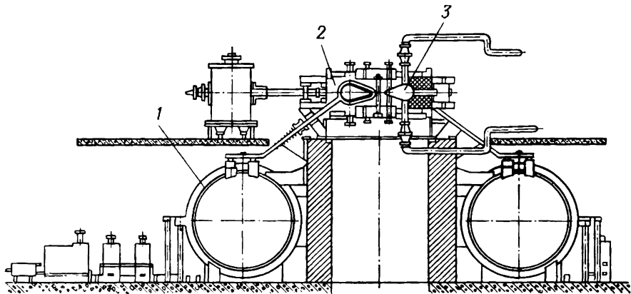
Fig. 7.4. T-14 tokamak design: 1) inductive accumulator of energy, 2) tokamak coils, 3) plasma.
