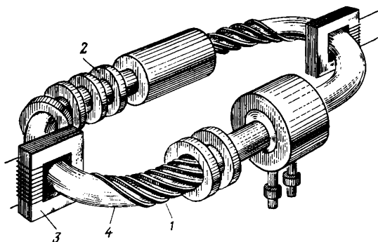
Fig. 4.7. Stellarator C: 1) helical winding, 2) longitudinal field coils, 3) ohmic heat transformer, 4) vacuum chamber.
