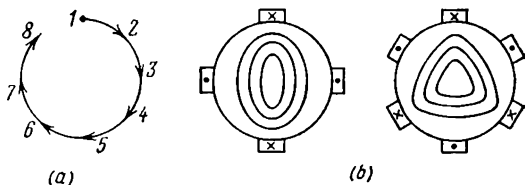
Fig. 4.6. (a) Rotation of magnetic field lines in a stellarator and (b) magnetic surfaces of stellarators with two and three pairs of helical conductors.
