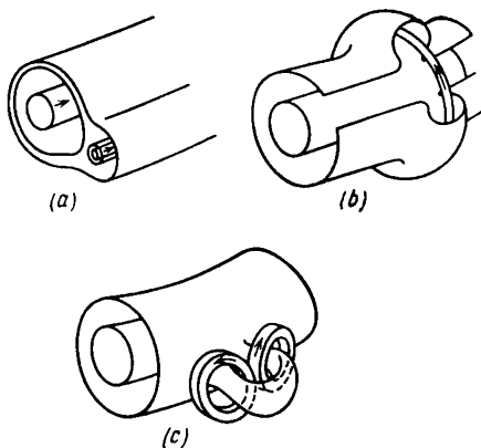
Fig. 6.9. Different types of divertor: (a) poloidal, (b) toroidal, and (c) bundle divertor.
