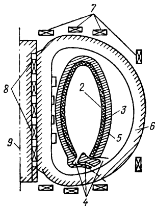
Fig. 11.2. Schematic diagram of a tokamak reactor: 1) plasma, 2) first wall, 3) blanket, 4) divertor space, 5) radiation shield, 6) toroidal magnetic field windings, 7) control and divertor windings, 8) inductor windings, 9) torus axis.
