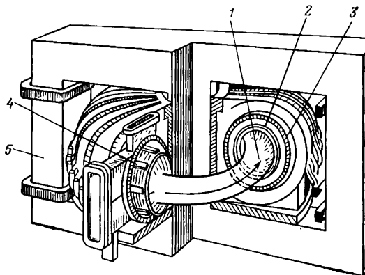
Fig. 5.2. Schematic diagram of a tokamak: 1) plasma, 2) stainless steel chamber, 3) copper casing, 4) transverse field winding, 5) transformer for exciting plasma current.
