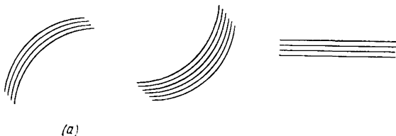
Fig. 3.7. Instability criterion for plasma confinement by a magnetic field: (a) unstable configuration, (b) stable configuration, and (c) neutral configuration.
