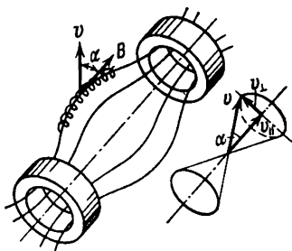
Fig. 3.1. Magnetic mirror trap. If the particle velocity in the middle of the trap forms a large angle with the direction of the magnetic field, the particle is reflected from magnetic mirrors and is confined in the trap. If the angle is too small, the particle falls into the "loss cone" and leaves the trap.
