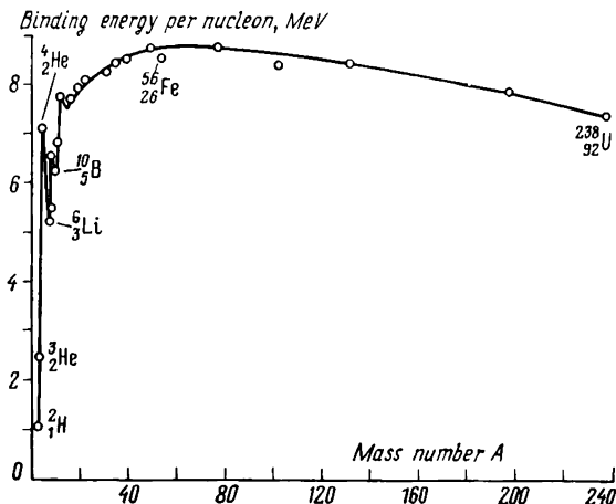
Fig. 1.1. Binding energy per nucleon vs. mass number A .
