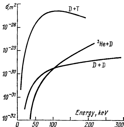
Fig. 1.2. Fusion reaction cross-section as a function of the energy of projectile nucleus.
