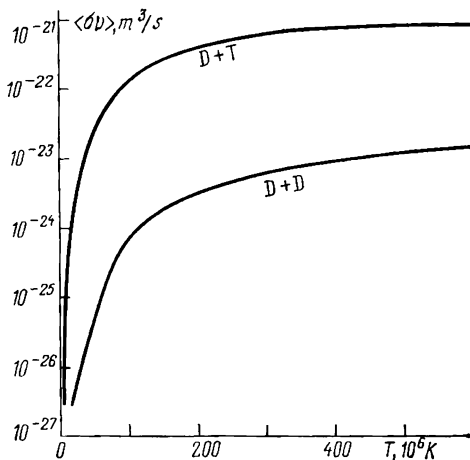
Fig. 1.3. Temperature dependence of the quantity \langle \sigma v \rangle , which determines the fusion reaction rate.
