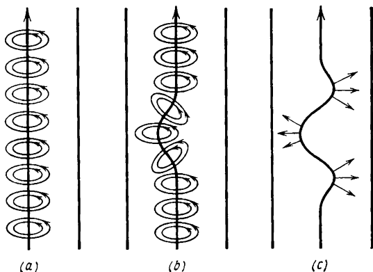
Fig. 2.3. Kink instability. A kink (b) appearing in a straight current-carrying plasma column (a) produces an excess magnetic field tending to make the kink more severe (c).
