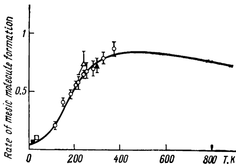
Fig. 10.1. Temperature dependence of the rate of formation of mesic molecules \text{D}\mu\text{D} . The symbols show the results of different experiments. The solid line corresponds to the predicted values.
