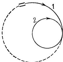
Fig. 3.4. Injection and capture of ions in a trap, based on the dissociation of molecular ions: 1) molecular ion trajectory, 2) atomic ion trajectory.
