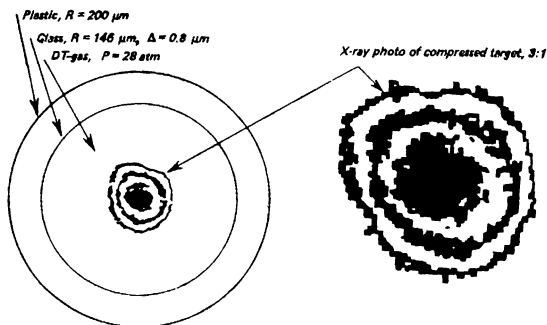
Fig. 9.5. Compression of the target by a laser pulse in a cold piston experiment.
