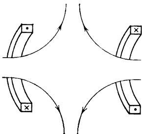
Fig. 3.8. Magnetic trap of cusp configuration.
