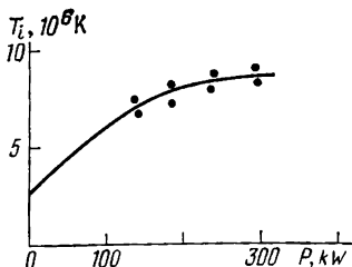
Fig. 6.7. Temperature to which ions are heated in a plasma as a function of the beam power.
