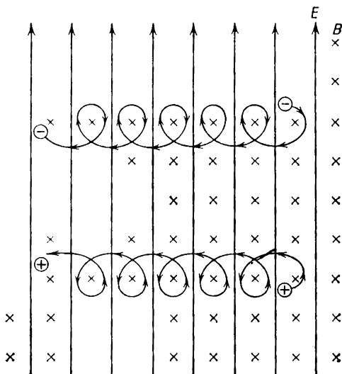
Fig. 1.6. Drift of charged particles in crossed electric and magnetic fields.
