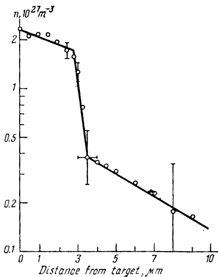
Fig. 9.3. Plasma density vs. distance from the target surface.
