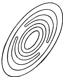
Fig. 8.2. Formation of "islands" in the stellarator's magnetic field structure near a magnetic surface for which the rotation angle of the induction lines is i \rightarrow 1/2 .
