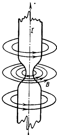
Fig. 2.2. Sausage-like instability. The plasma column is disrupted by increased magnetic field pressure in the region of constriction.
