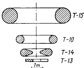
Fig. 7.5. Comparison of plasma size in Soviet tokamaks.
