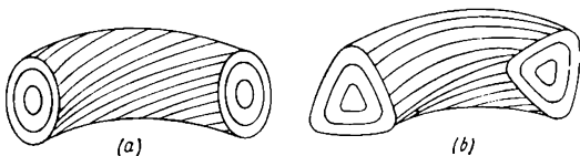
Fig. 8.1. Magnetic field structure in (a) a tokamak and (b) a stellarator.
