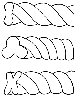
Fig. 5.5. The plasma assumes the form of a two-, three- or four-threaded helix.
