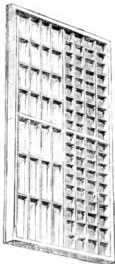
LABOR SAVING RULE CASE.
