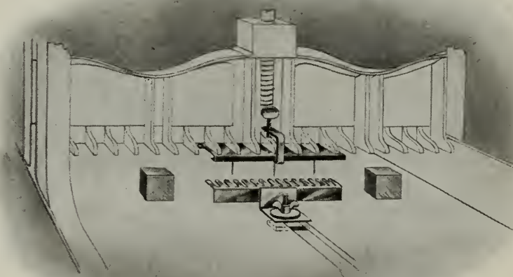
Challenge Book Stabber Adjusted on a Paper Cutter Ready for Use.
