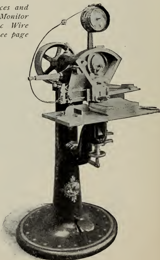
No. 0 Monitor Wire Stitcher.
