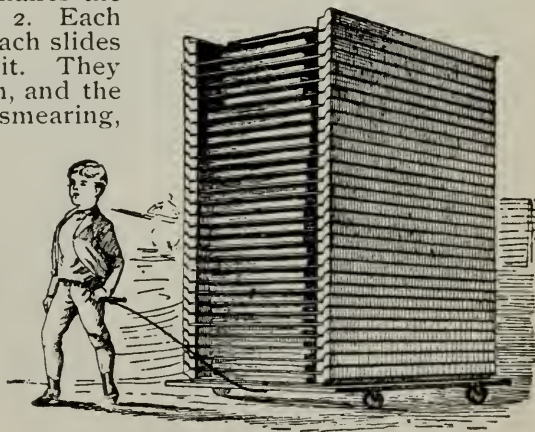
Fig. 1. Köerner's Racks on Printer's Truck.
