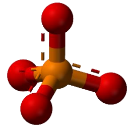
A Phosphate Molecule
